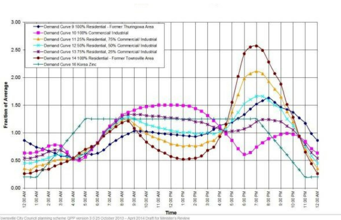
Figure 6.4.11.1 - Water Demand Daily Diurnal Variations
